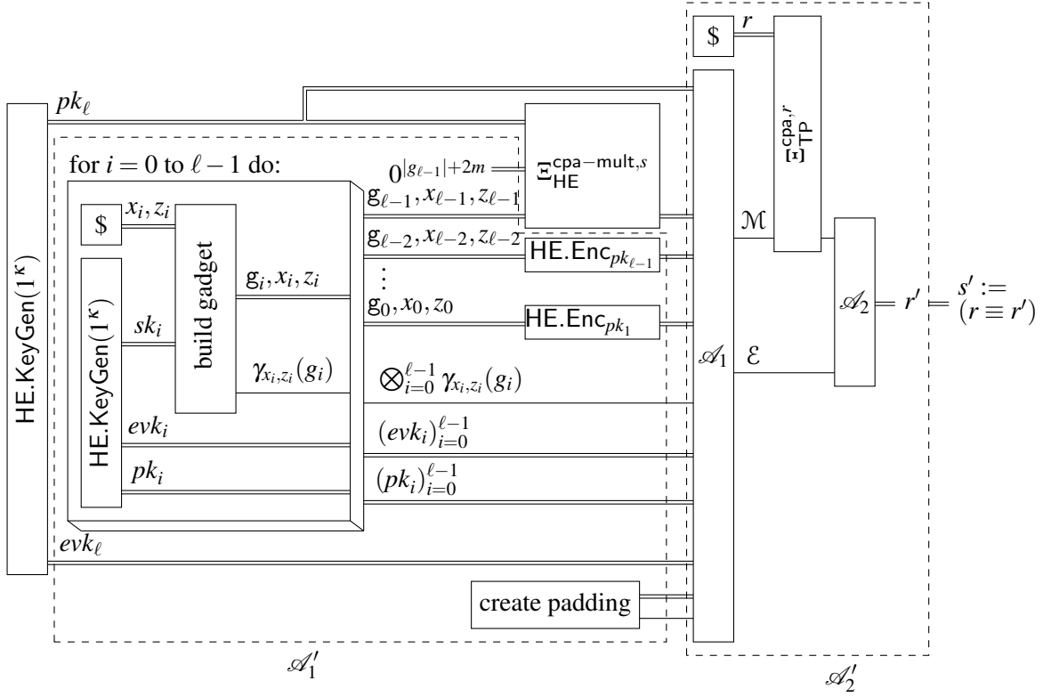
Figure 3: A strategy for the game \text{PubK}_{\mathcal{A}', \text{HE}}^{\text{cpa-mult}}(\kappa) , using an adversary \mathcal{A} for \text{PubK}_{\mathcal{A}, \text{TP}^{(\ell)}}^{\text{cpa}}(\kappa) as a subroutine. All the wires that form an input to \mathcal{A}_1 together form the evaluation key and public key for \text{TP}^{(\ell)} or \text{TP}^{(\ell-1)} , depending on s . Note that \Xi_{\text{TP}}^{\text{cpa}, r} = \Xi_{\text{TP}^{(\ell)}}^{\text{cpa}, r} = \Xi_{\text{TP}^{(\ell-1)}}^{\text{cpa}, r} , so \mathcal{A}_2 can run either one of these independently of s (i. e., without having to query the challenger). The “create padding” subroutine generates dummy gadgets for \ell up to L - 1 , as described in the definition of \mathcal{A}_1 .
