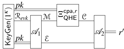
Figure 1: [16, reproduced with permission of the authors] The quantum CPA indistinguishability experiment \text{PubK}_{\mathcal{A}, \text{QHE}}^{\text{cpa}}(\kappa) . Double lines represent classical information flow, and single lines represent quantum information flow. The adversary \mathcal{A} is split up into two separate algorithms \mathcal{A}_1 and \mathcal{A}_2 , which share a working memory represented by the quantum state in register \mathcal{E} . For the definition of \Xi_{\text{QHE}}^{\text{cpa}, r} , see step 3 in Definition 2.1.
