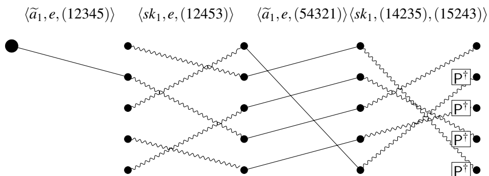
Figure 4: Structure of the (first half of the) gadget, with measurements, coming from the 5-permutation branching program for the OR function on the input (0, 0) . The example program’s instructions are displayed above the permutations. The solid lines correspond to Bell measurements, while the wavy lines represent EPR pairs.
