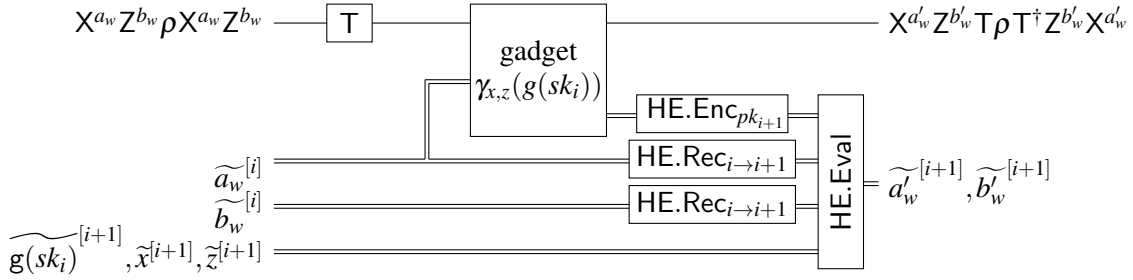
Figure 2: The homomorphic evaluation of the (i + 1) th T gate of the circuit. The gadget is consumed during the process. After the use of the gadget, the evaluator encrypts his own classical information (including measurement outcomes) in order to use it in the homomorphic computation of the new keys. HE.Eval evaluates this fairly straightforward computation that consists mainly of looking up values in a list and adding them modulo 2. Note that \widetilde{sk}_i^{[i+1]} , needed for the decryption procedures, is contained in the evaluation key and that the keys of the wires that are not shown are also reencrypted.
