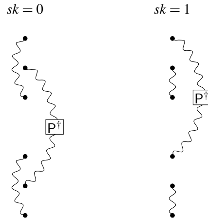
Figure 7: The two possible gadgets \Gamma(sk) that TP.GenGadget might generate for TOY.Dec. Effectively, a gadget consists of 2GH(\text{TOY.Dec}) EPR-pairs, ordered in a way that depends on sk . Some EPR-pairs have an additional (P^\dagger \otimes I) transformation applied to them. The evaluator’s input c determines whether or not the input qubit is teleported through such a transformation, but an evaluator is unable to tell whether it is.
