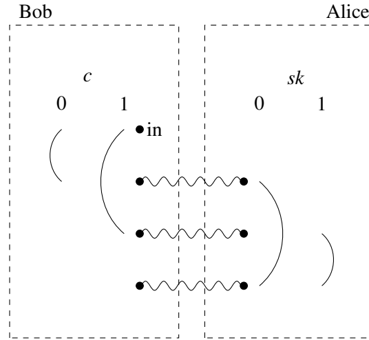
Figure 5: Garden-hose protocol for TOY.Dec. The snaky lines represent the EPR-pairs that form the resources to the protocol. The bended lines represent Bell measurements that Bob and Alice perform dependent on their inputs. For example, if c = 0 and sk = 0 , the qubit starting at “in” is teleported through the first EPR-pair by Bob, then back through the third EPR-pair by Alice. It comes out on the bottom location on Bob’s side.
