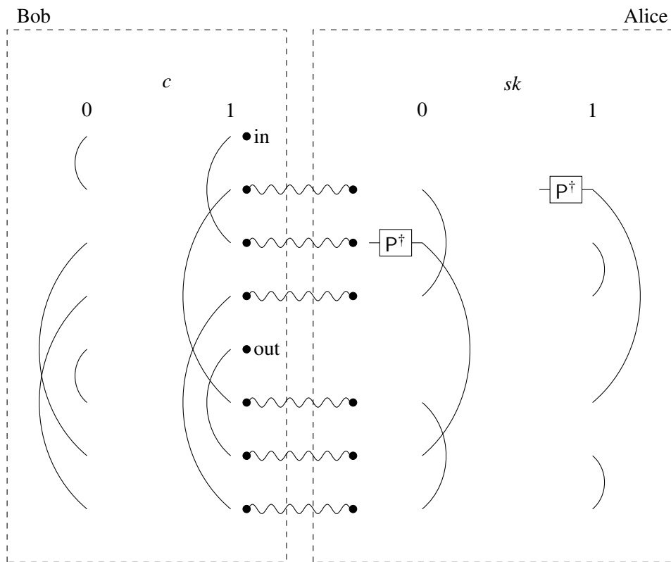
Figure 6: Removal of a possible P error using two copies of the garden-hose protocol for TOY.Dec. For example, if c = 0 and sk = 1 , the qubit is teleported through EPR pairs 1 and 4, with a P^\dagger applied to it by Alice in between. The input qubit always ends up on position “out.”
