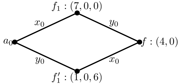
Figure 2: The (7, 0, 0) and (1, 0, 6) neighbors of a (4, 0) function.
