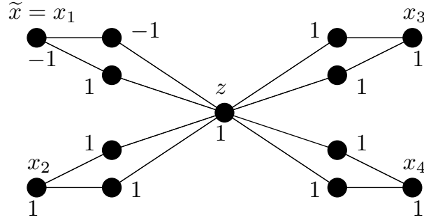
Figure 3: The neighborhood of z . The variables are labeled with the assignment d_i gives them. Note that the assignment of z agrees with all but one of its neighbors and all but one of the x_j . Further, the two variables which disagree with z are adjacent.
